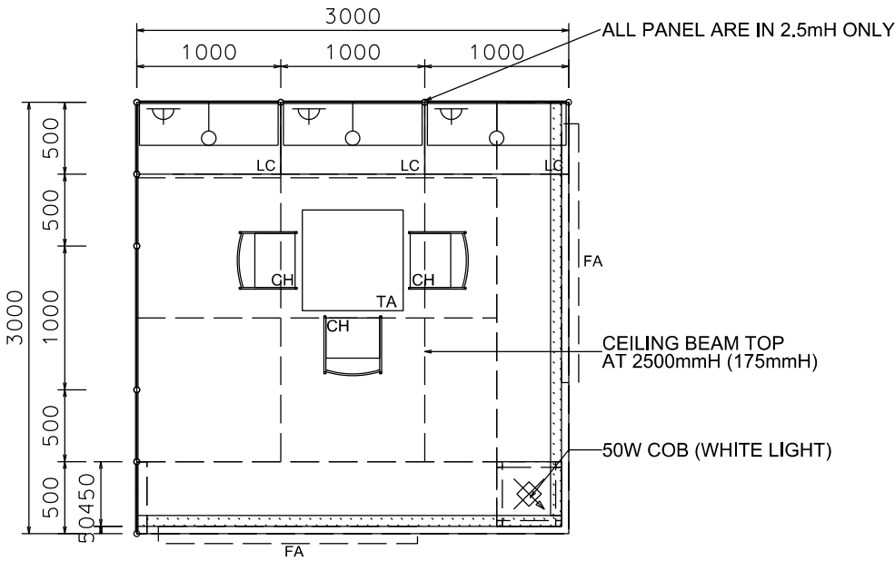
PLAN
