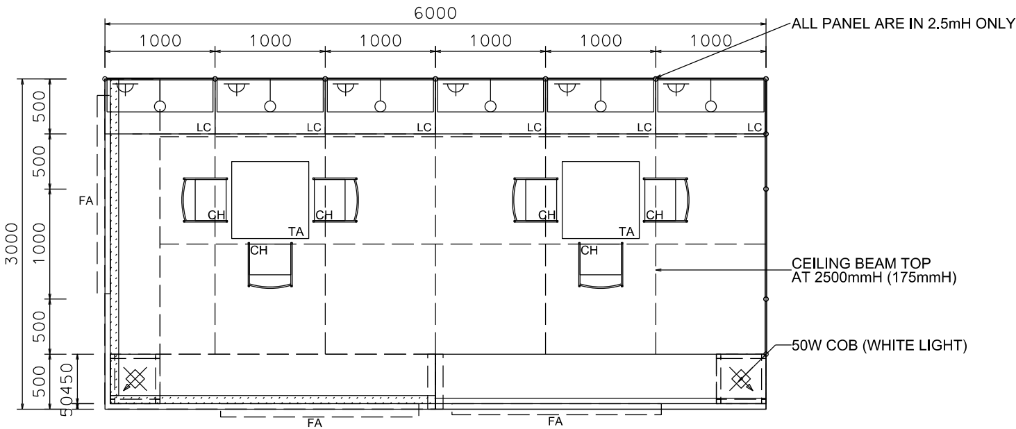
PLAN
