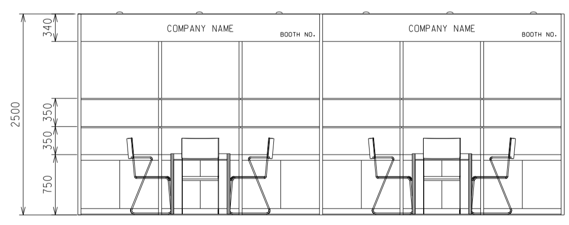
ELEVATION 6M(W) X 3M(D) X 2.5M(H) Right Corner Booth A
