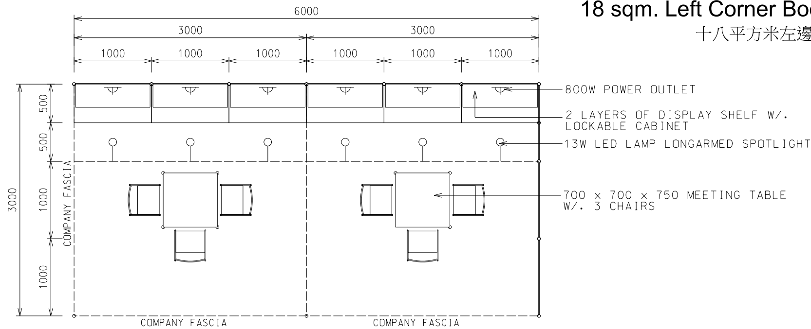
PLAN 6M(W) X 3M(D) X 2.5M(H) Left Corner Booth A
