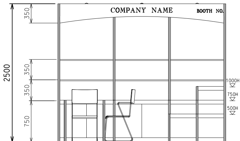
ELEVATION 3M(W) X 3M(D) X 2.5M(H) Left Corner Booth B
