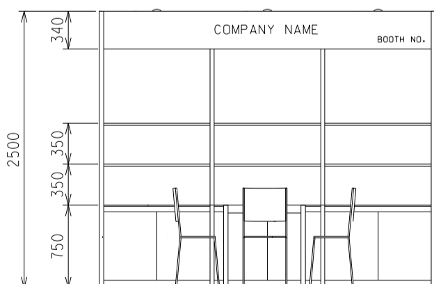
ELEVATION 3M(W) X 3M(D) X 2.5M(H) Right Corner Booth A
