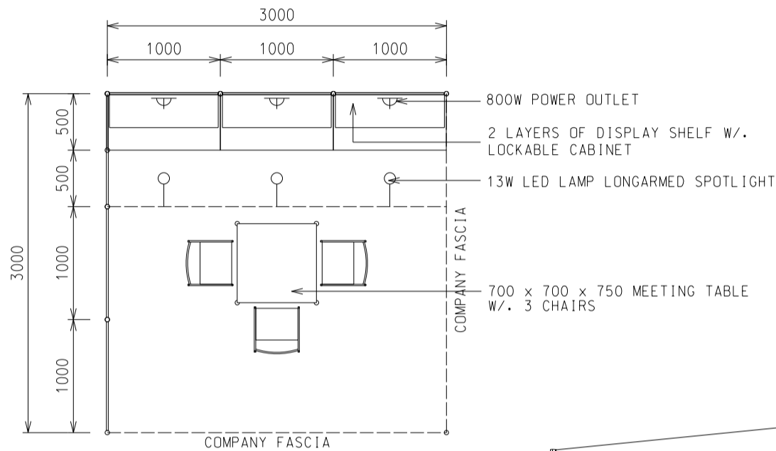
PLAN 3M(W) X 3M(D) X 2.5M(H) Right Corner Booth A
