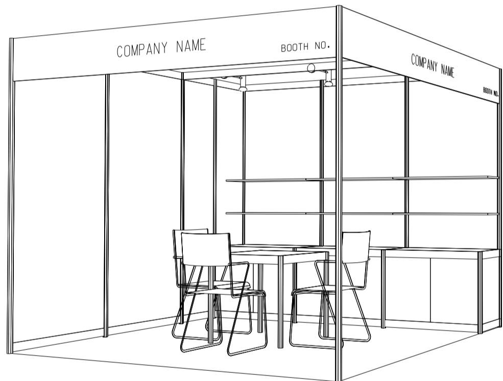
PERSPECTIVE 3M(W) X 3M(D) X 2.5M(H) Right Corner Booth A
