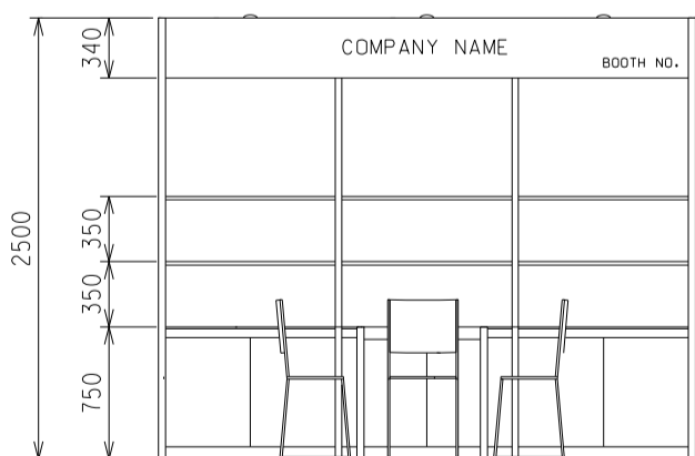
ELEVATION 3M(W) X 3M(D) X 2.5M(H) Left Corner Booth A
