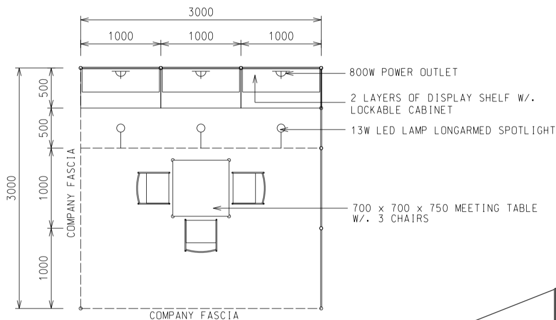
PLAN 3M(W) X 3M(D) X 2.5M(H) Left Corner Booth A
