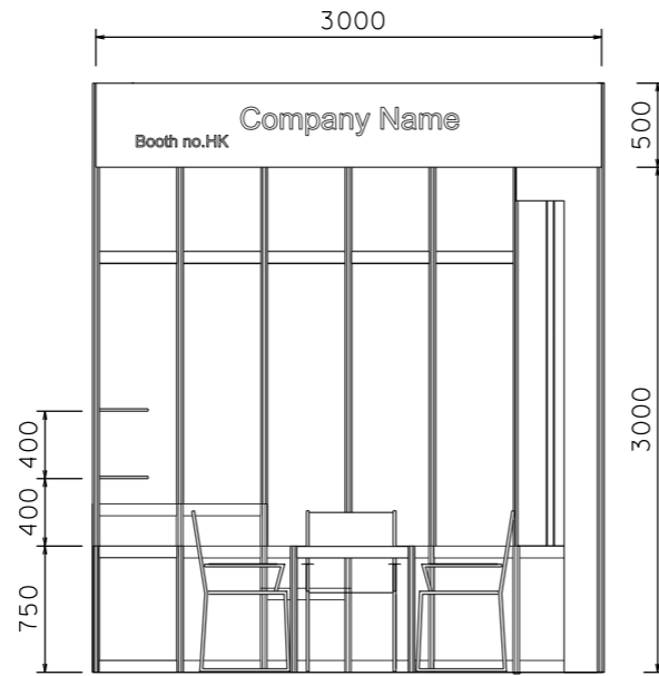
SIDE ELEVATION
